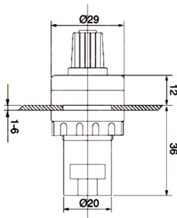
Dimension structure drawing
